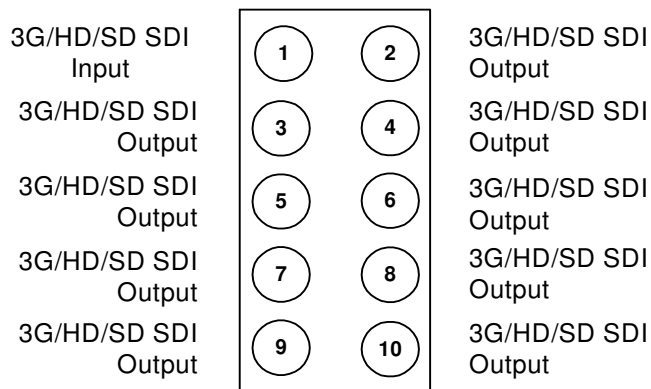
Figure 3. BNC Designations for the Card Rear Module RM-9001-A or 8310-RM-100
