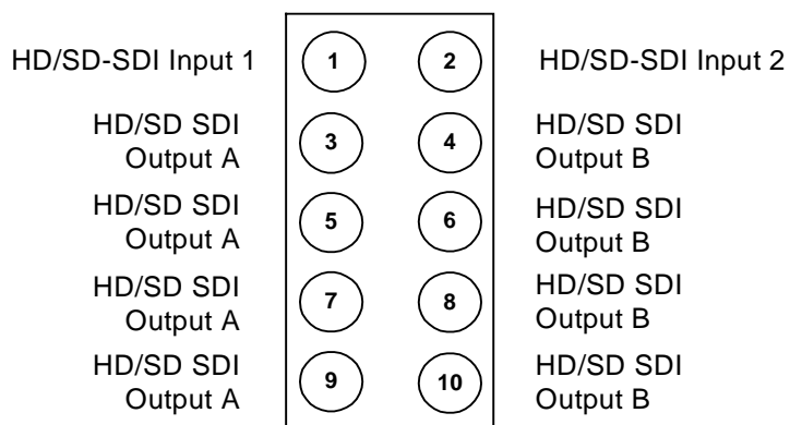
Figure 3. BNC Designations for the Card Rear Module RM-9003-A or 8310-RM-100
