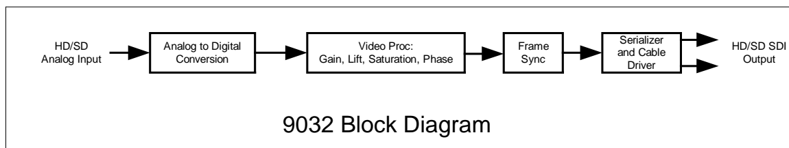
Figure 1. Simplified Block Diagram of 9032 Functions
