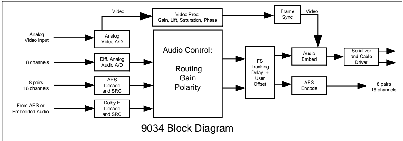
Figure 1. Simplified Block Diagram of 9034 Functions
