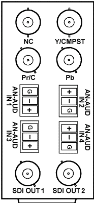
RM-9034-B
