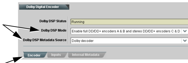
Figure 2 Example Routing and Dolby Re-Encode Processing (Sheet 2 of 4)
