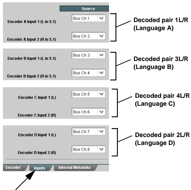
Figure 2 Example Routing and Dolby Re-Encode Processing (Sheet 3 of 4)
