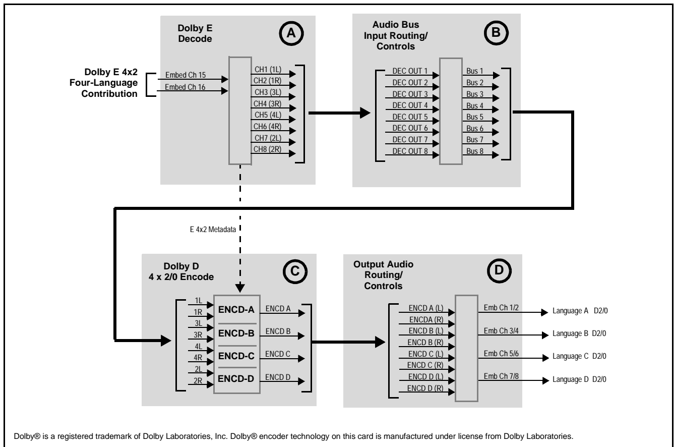
Figure 2 Example Routing and Dolby Re-Encode Processing (Sheet 1 of 4)
