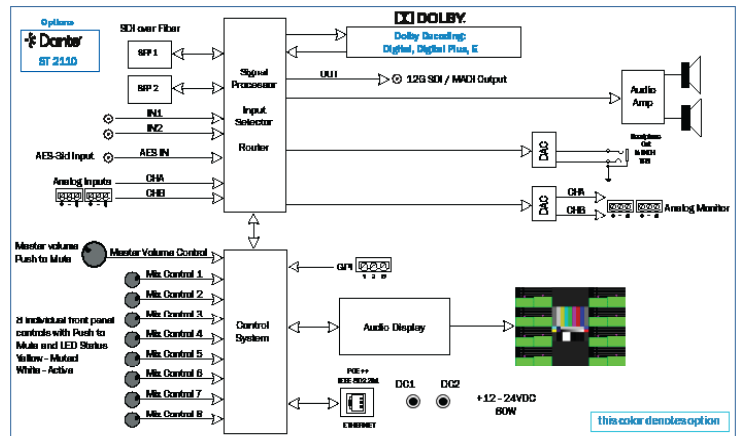
ARIA AUD-MON-H 1RU Audio Monitor
